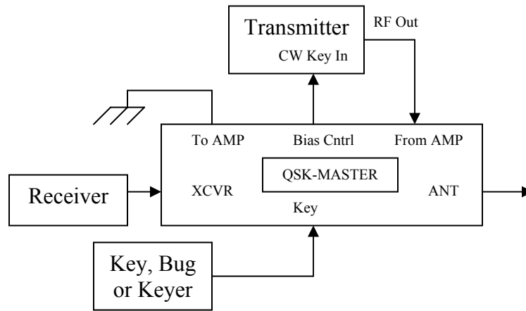
Figure 2: QSK-MASTER as Boat-Anchor T/R Switch
