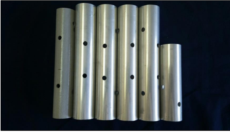
Coupling inserts. Leftmost is the fiberglass insulator for the top of the base mast section. Short one is 4-3/4" (120 mm) for the top section. The rest are 7-1/8" (182 mm) long. NOTE: SHORT COUPLER MAY BE PREINSTALLED IN TOP SECTION.
