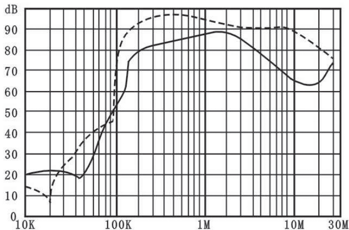
Attenuation Plot vs Frequency
