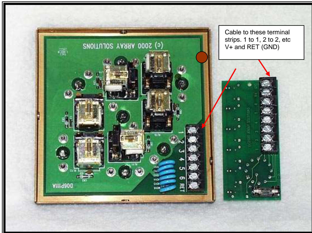
Figure 1: RATPak relay box and rotary controller boards
